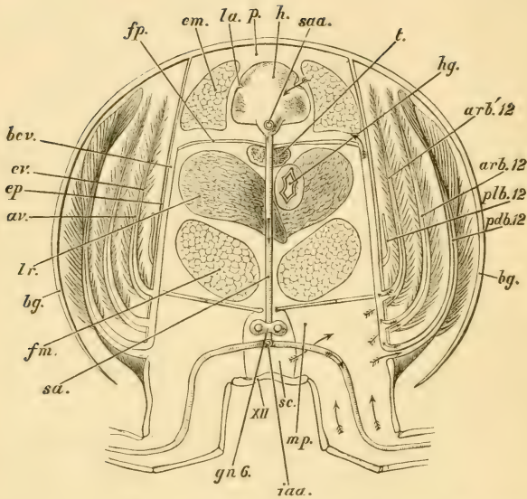
FIG. 15.— Astacus fluvialtilis .—A diagrammatic transverse section of the thorax through the twelfth somite, showing the course of the circulation of the blood ( \times 3 ). arb. 12 , the anterior or lower, and arb'. 12 , the posterior or upper arthrobranchia of the twelfth somite; av , afferent branchial vessel; bcv , branchio-cardiac vein; bg , branchiostegite; em , extensor muscles of abdomen; ep , epimeral wall of thoracic cavity; ev , efferent branchial vessel; fm , flexor muscles of abdomen; fp , floor of pericardium; gn. 6 , fifth thoracic ganglion; h , heart; hg , hind-gut; iaa , inferior abdominal artery, in cross section; la , lateral valvular apertures of heart; lv , liver; mp , indicates the position of the mesophragm by which the sternal canal is bounded laterally; p , pericardial sinus; pdb. 12 , podobranchia, and plb. 12 , pleurobranchia of the twelfth somite; sa , sternal artery; saa , superior abdominal artery; sc , sternal canal; t , testis; XII., sternum of twelfth somite. The arrows indicate the direction of the blood flow.
